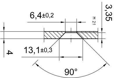
detail mounting hole track
